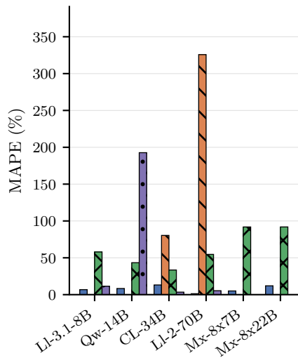
ITL Mean
