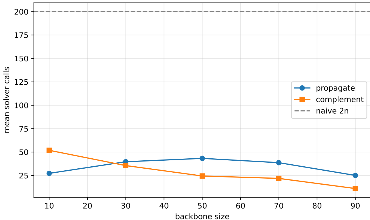
Calls against backbone size, CBS instances with 100 variables
