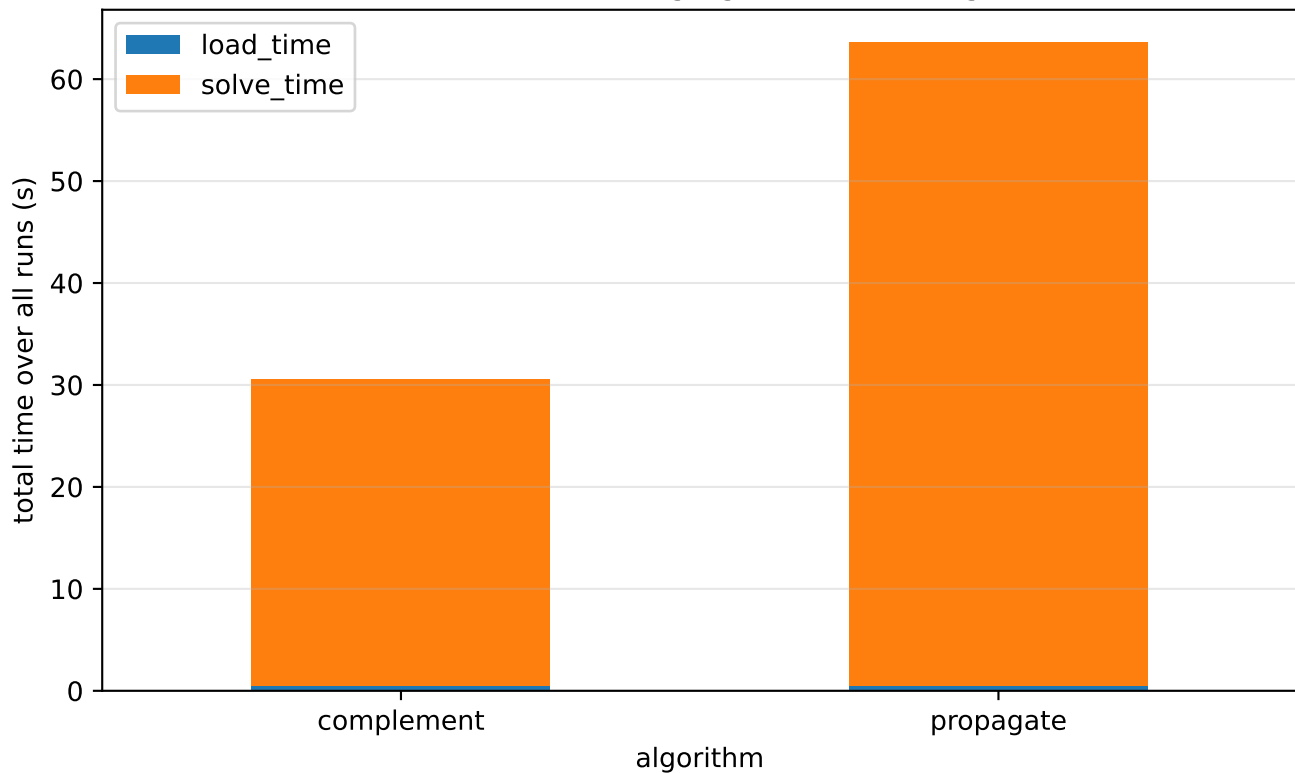
Runtime, loading against searching
