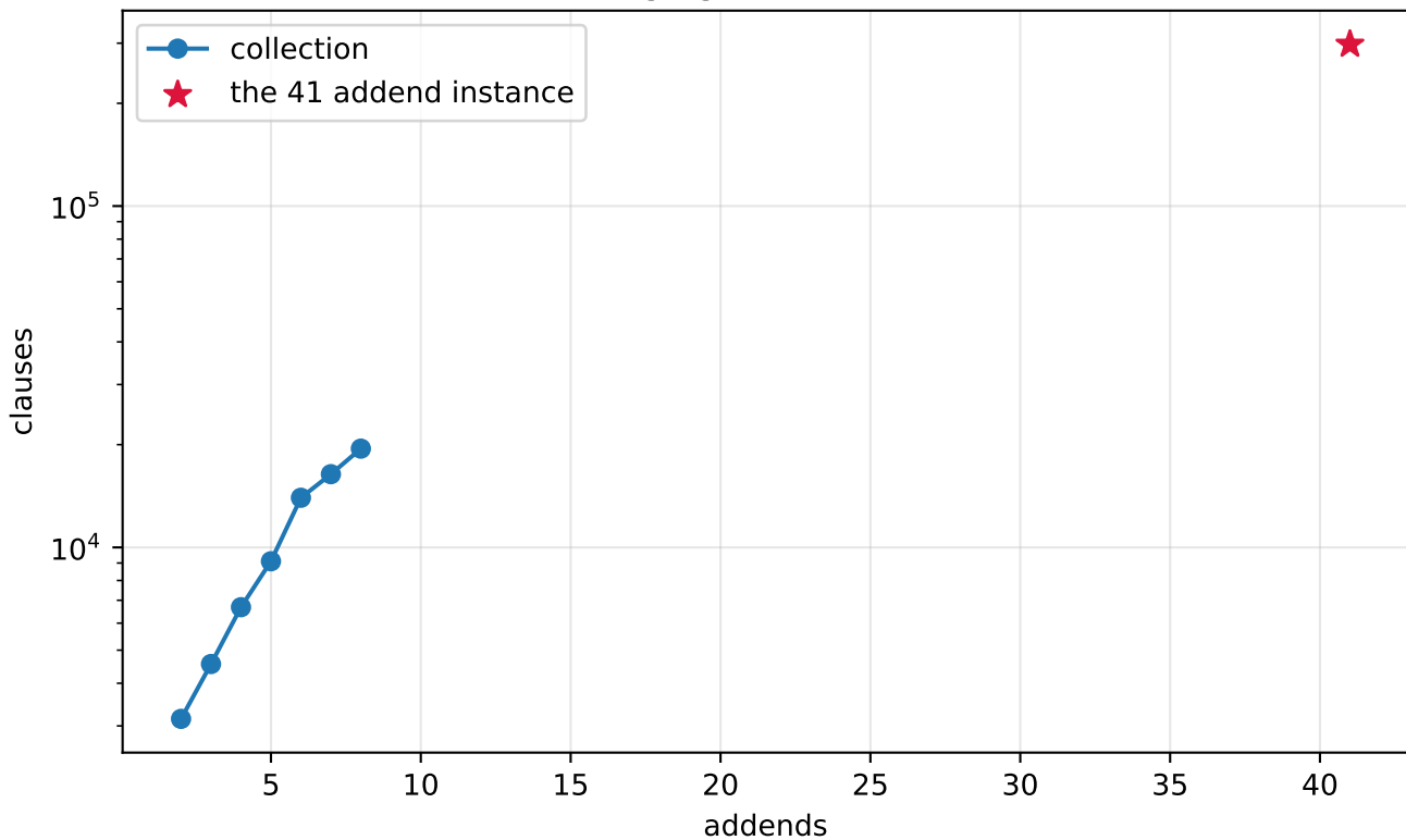
Size of the encoding against the number of addends
