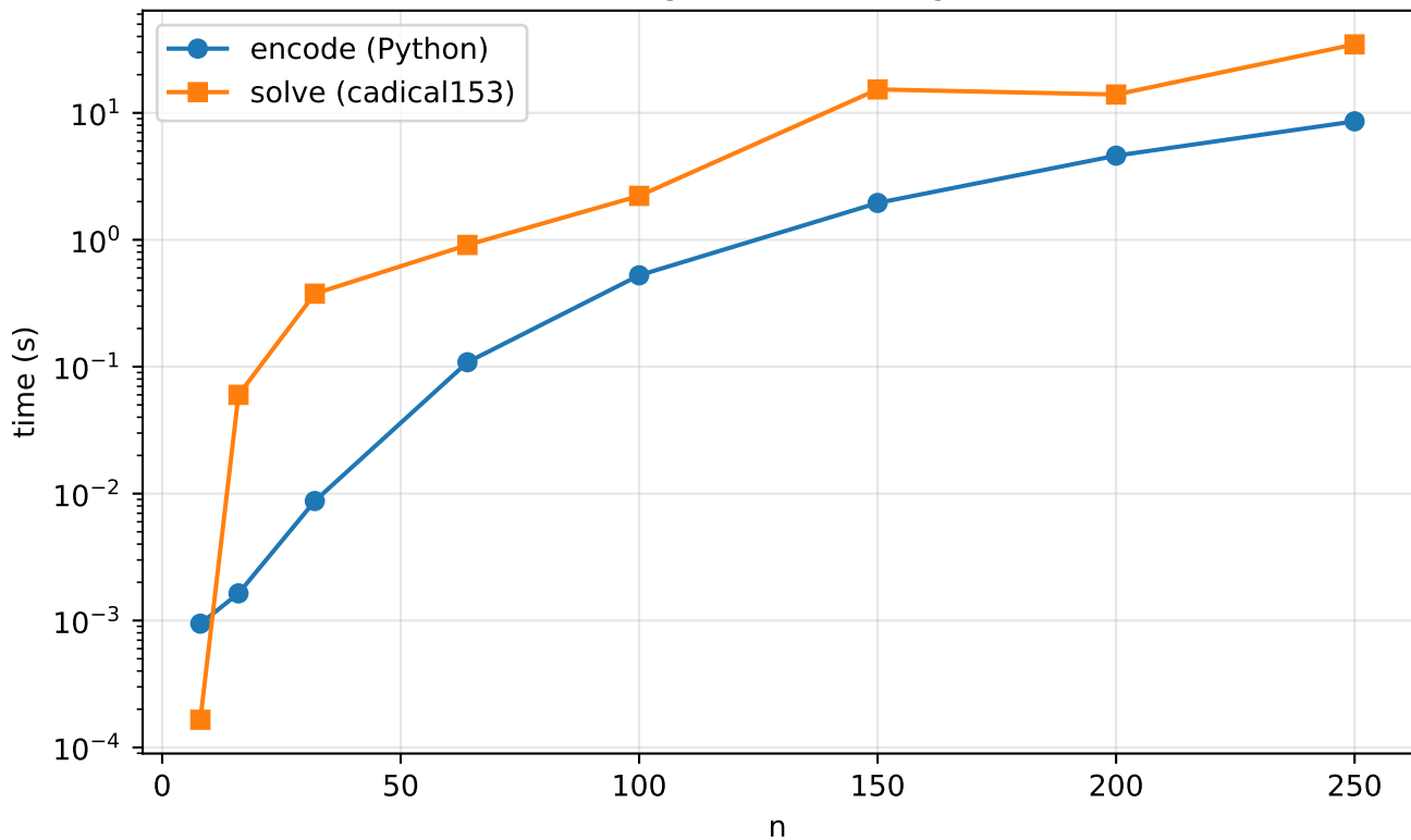
Encoding cost vs solving cost
