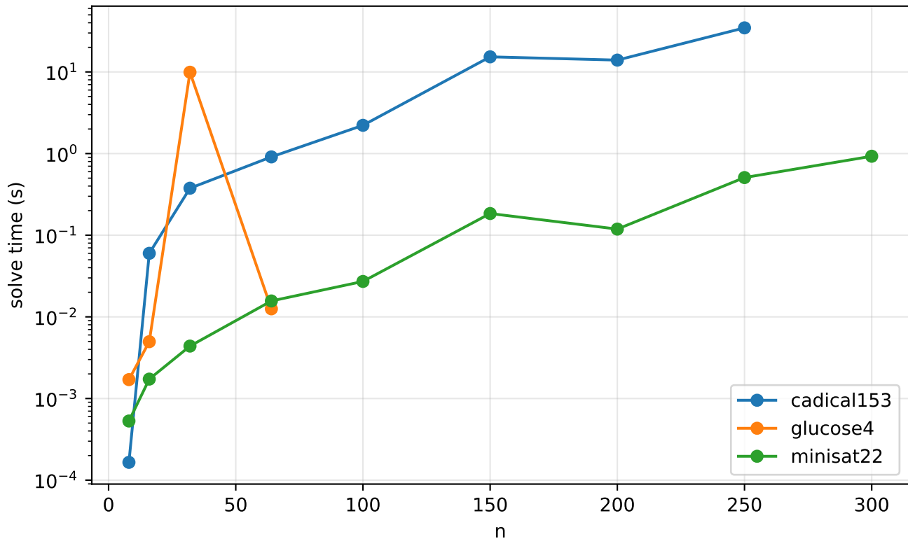
Solve time vs n
