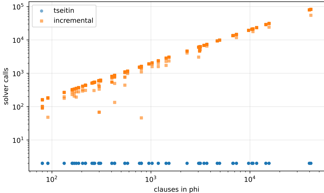
Number of solver calls
