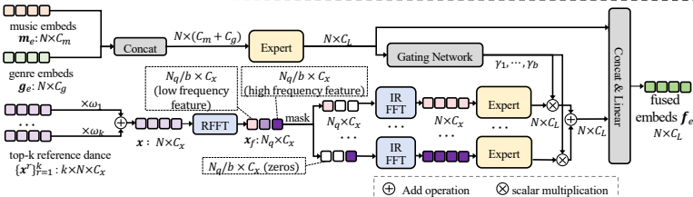
(b) The Cadence MoE
