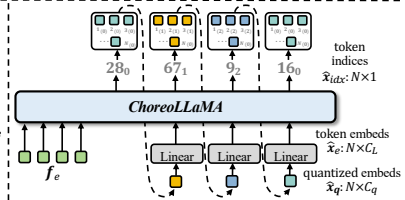
(c) The inference process of ChoreoLLaMA
