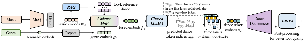
(a) The overall framework of ChoreoLLaMA
