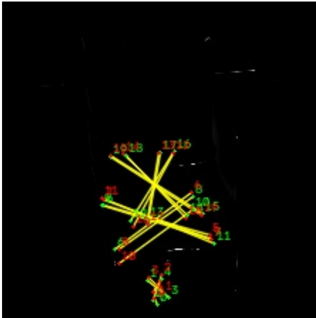
Fig. 8.4 MobilePose, VisCam_0029974 .
