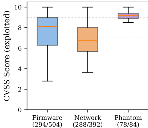
(b) By Attack Layer
