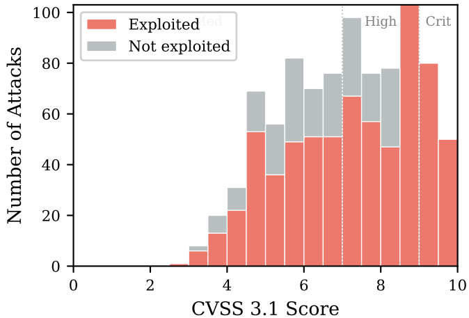
(a) Score Distribution
