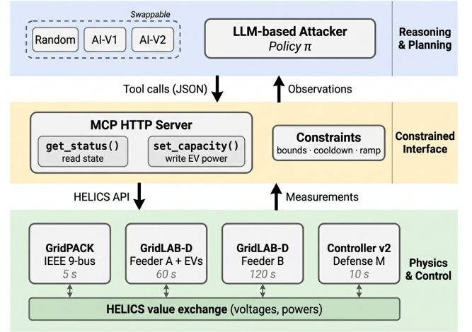
Figure 1: LLM-GridEval architecture. The co-simulation layer (bottom) runs the HELICS federation; the interface layer (middle) enforces schema-constrained primitives with validation; the cognitive layer (top) hosts swappable attacker policies.
