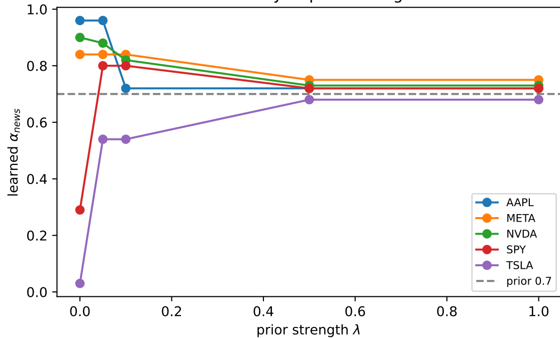
Sensitivity to prior strength
