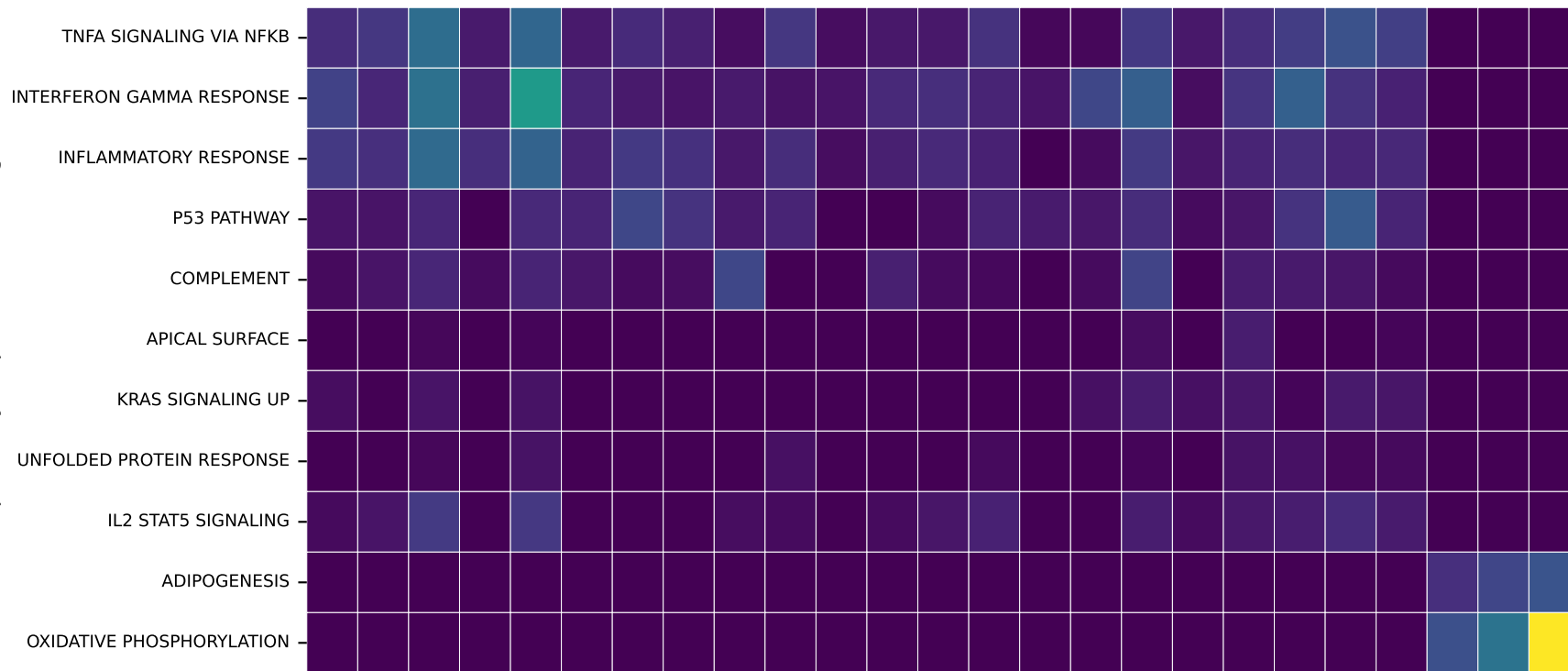
Leading-edge gene overlap: Hallmark vs Reactome (representative, padj<0.05 sets; both ranked on DESeq2 Wald stat)
