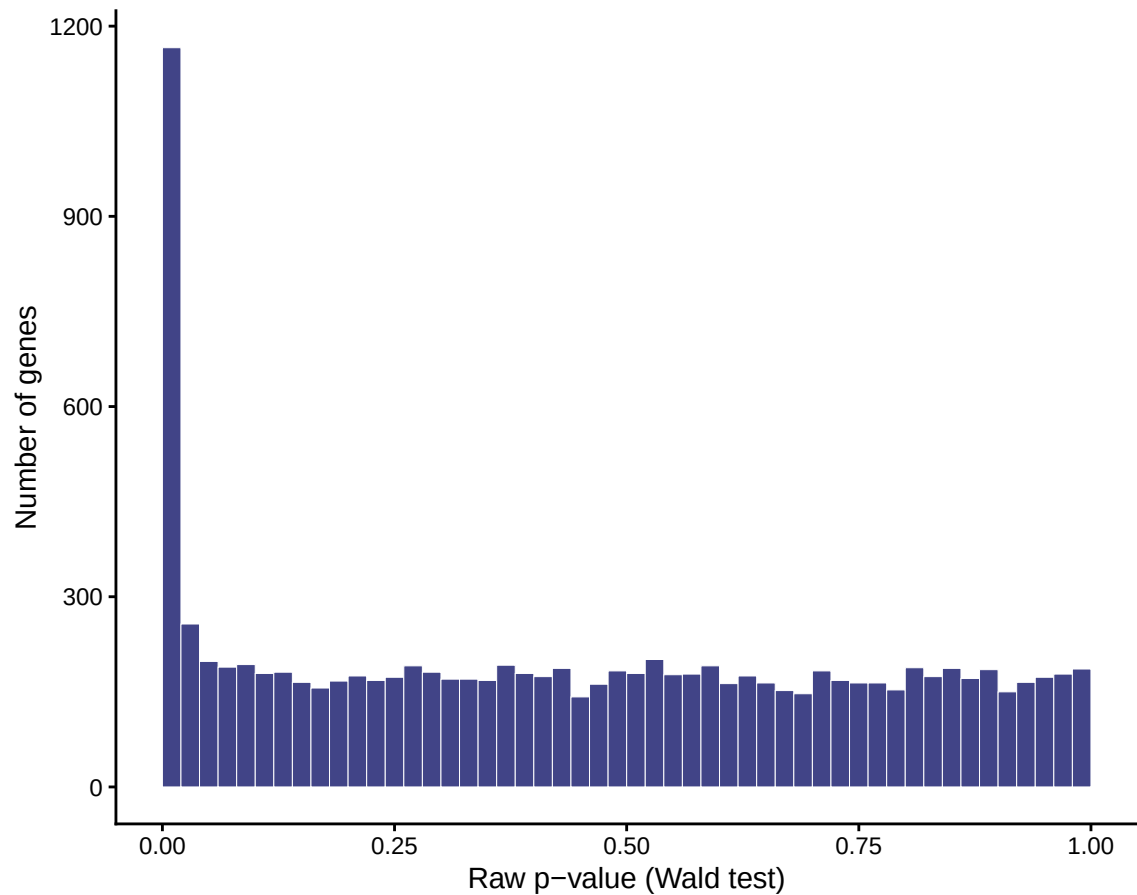
P-value distribution before BH adjustment
