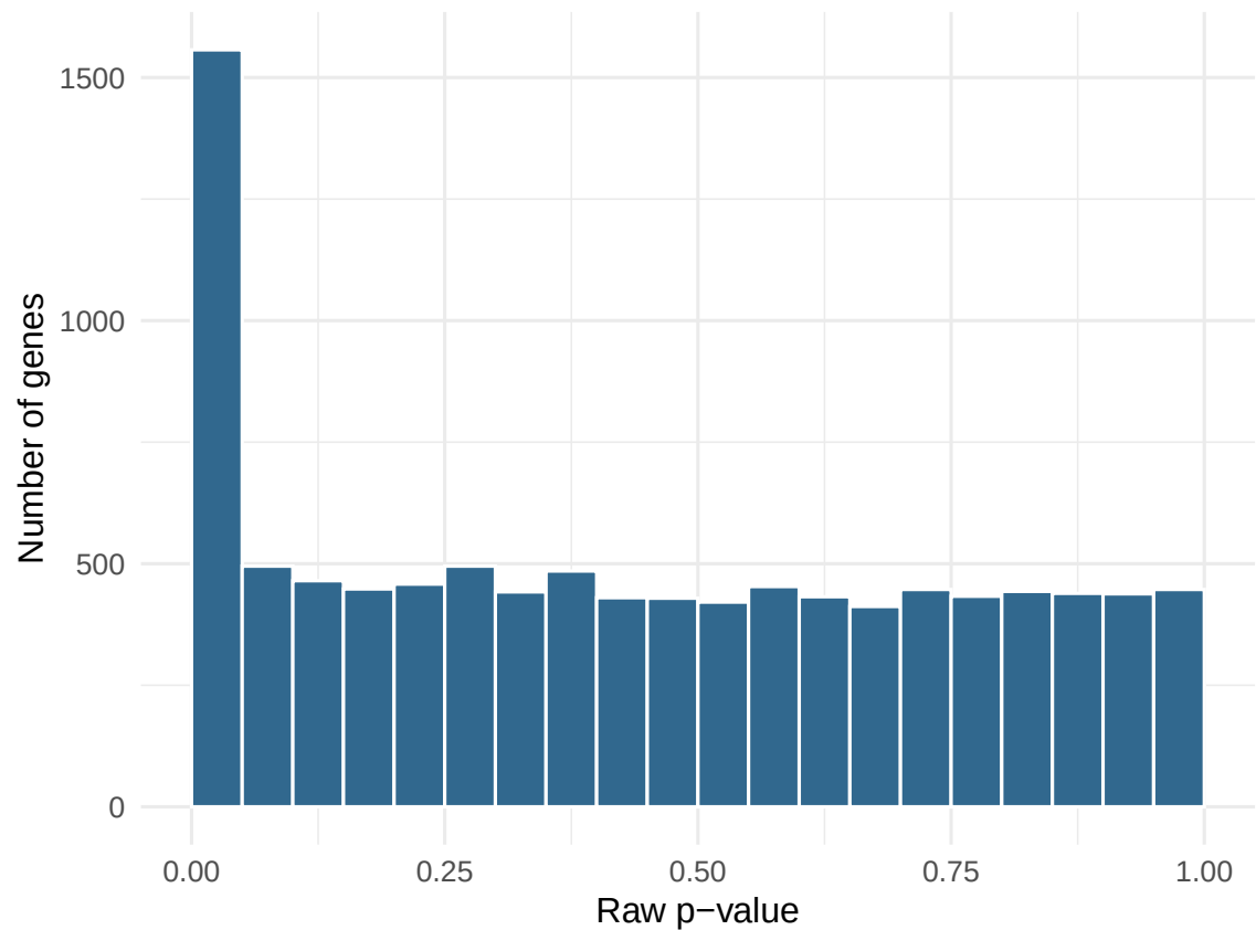
P-value histogram, Wald test (condition treated vs control) Primary contrast, sample_01 excluded
