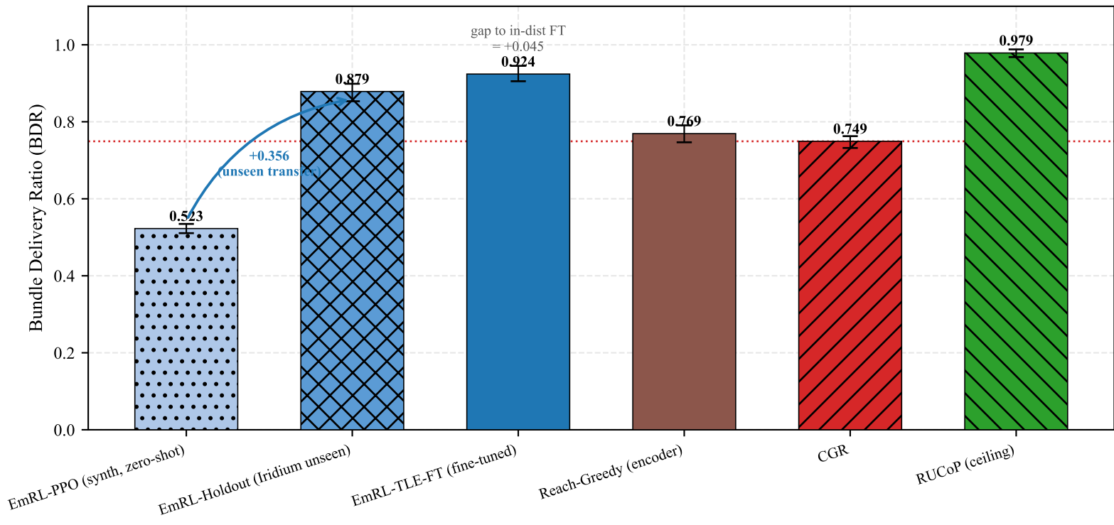
Leave-one-out generalization — Iridium-NEXT held out of training (5 seeds \times 150 episodes; held-out model never saw Iridium)
