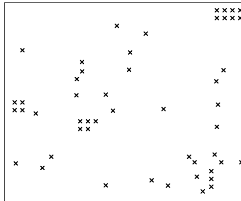
Drill Map: x 0.300mm / 0.0118" (50 holes)
