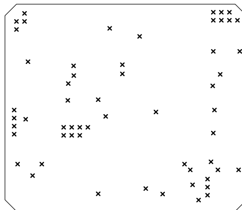
Drill Map: x 0.300mm / 0.0118" (57 holes)
