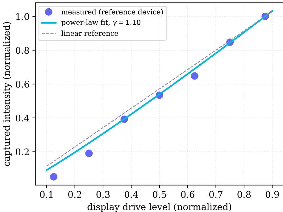
Figure 3. Optical channel transfer curve
