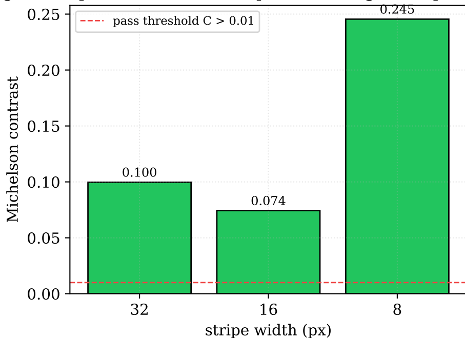
Figure 4. Spatial contrast (MTF points) through the optical channel
