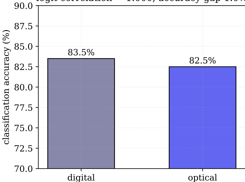
Figure 8. One neural layer 256 \rightarrow 64 \rightarrow 10 logit correlation = 1.000, accuracy gap 1.0%
