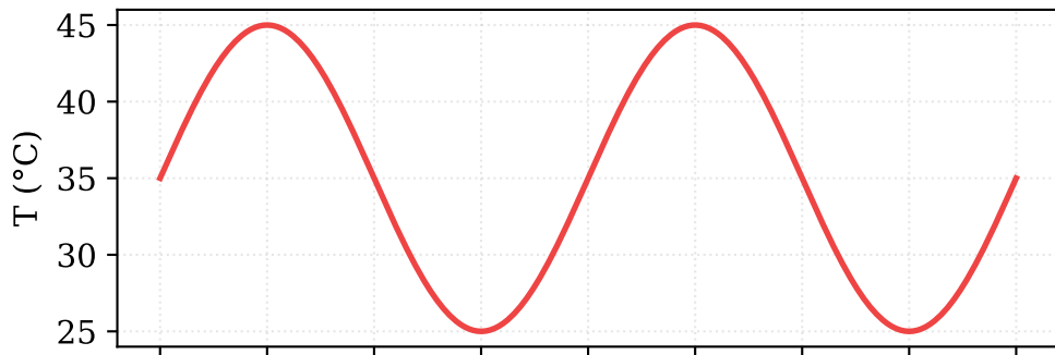
Figure 11. Thermal grating \Lambda = 4 \text{ mm} \rightarrow refractive gradient
