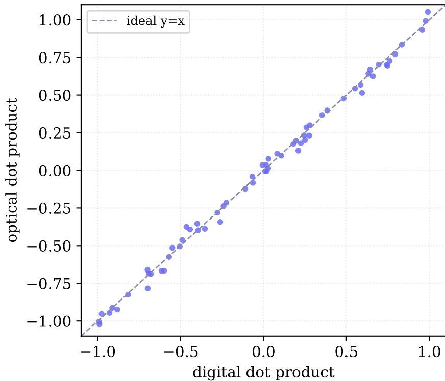
Figure 7. Optical vs digital MatVec Pearson r = 0.998 (simulation)
