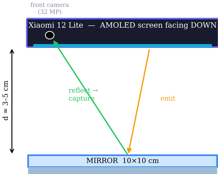
Figure 1. The OLED-mirror-camera optical channel (side view)
