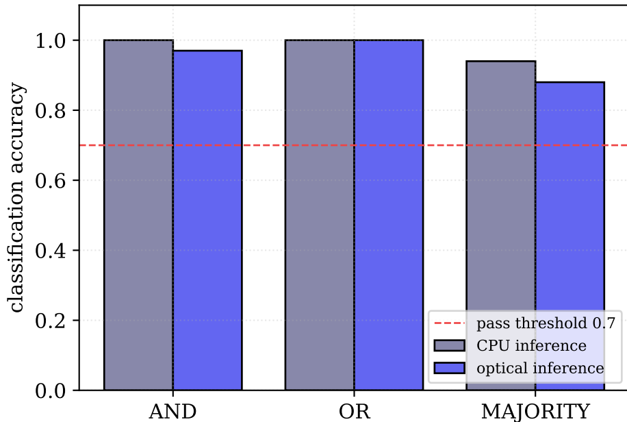
Figure 18. Optically-evaluated perceptron after training (model of stage72)
