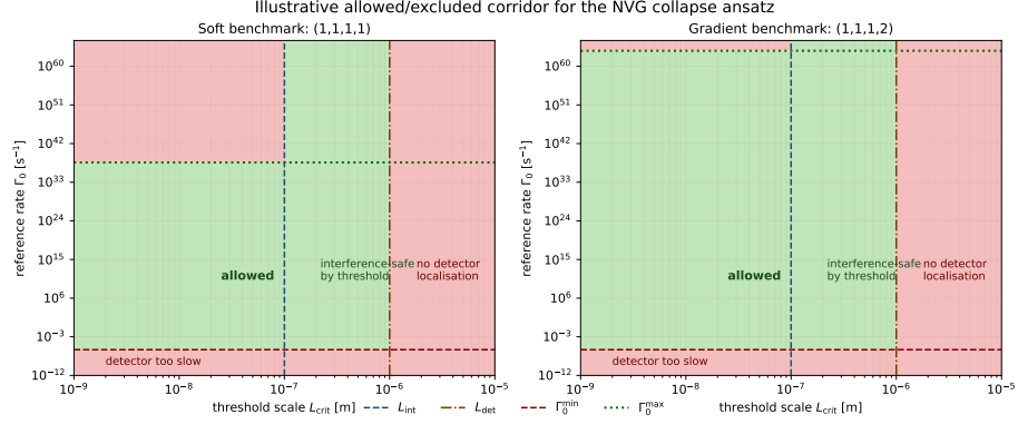
Figure 1: Illustrative allowed and excluded regions in the (L_{crit}, \Gamma_0) plane for the two benchmark NVG collapse ansaetze. Green indicates benchmark-compatible regions; red indicates regions excluded either because microscopic interferometry would be spoiled or because detector localisation would be too slow.
