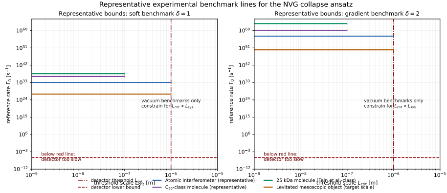
Figure 2: Representative benchmark lines in the (L_{crit}, \Gamma_0) plane for atomic interferometry, molecule interference, and mesoscopic superposition targets. The red detector line is a lower bound required for fast localisation in a macroscopic detector, while colored horizontal lines show approximate upper bounds from preserving interference in representative vacuum experiments.
