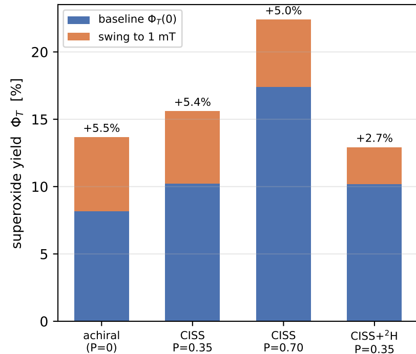
(c) baseline + magnetic swing
