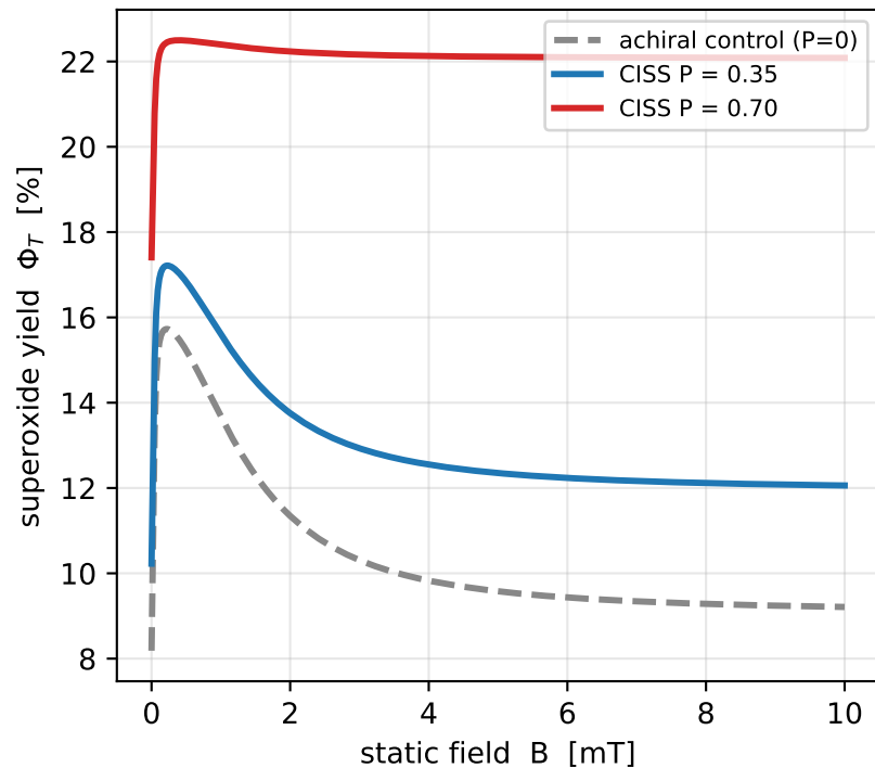
(a) chirality raises baseline ROS
