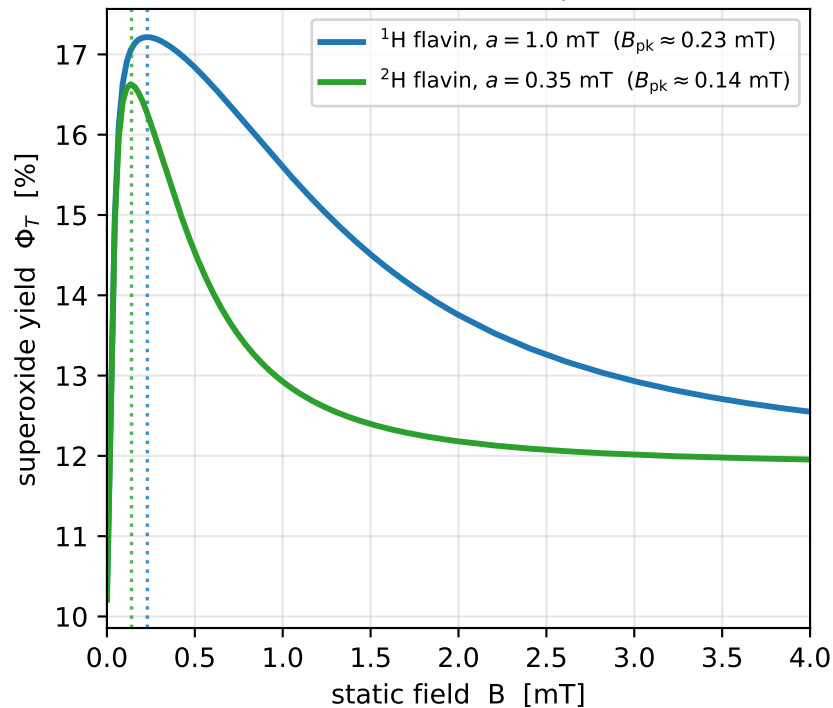
(b) isotope test: B_{pk} \propto a
