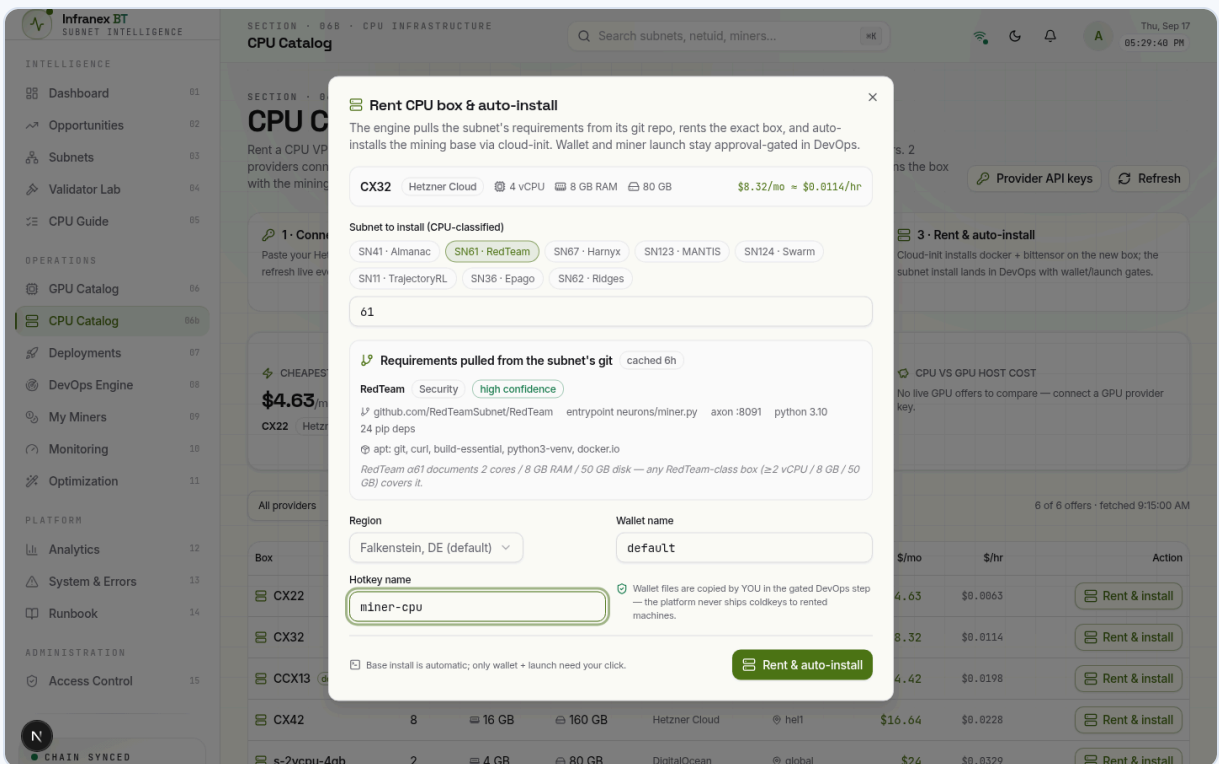
Figure 6. The rent dialog, fully filled for the worked example — example data . CX32 pinned at top, SN61 selected from the chips, the git-pulled requirements panel showing high confidence, region Falkenstein, wallet default, hotkey miner-cpu.
