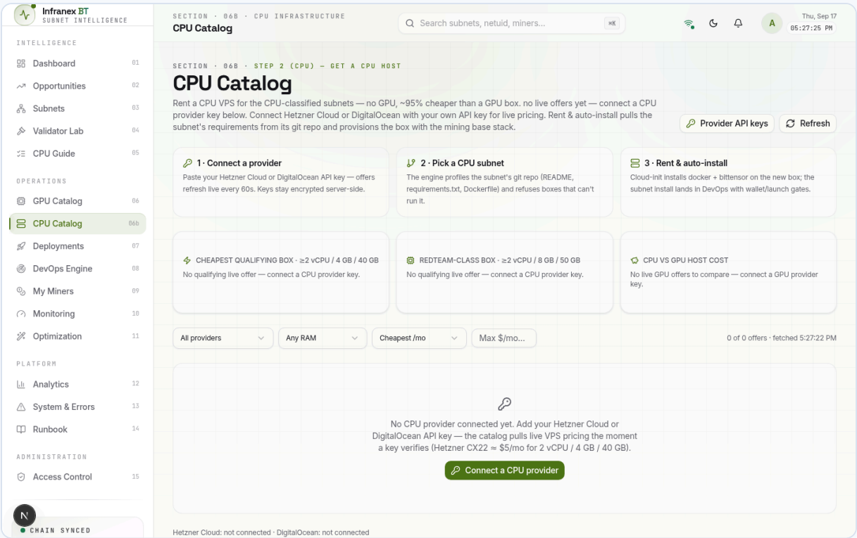
Figure 4. The catalog before any key is connected — the empty state names the missing piece and the expected price (Hetzner CX22 ≈ $5/mo) so you can tell honesty from a bug.
