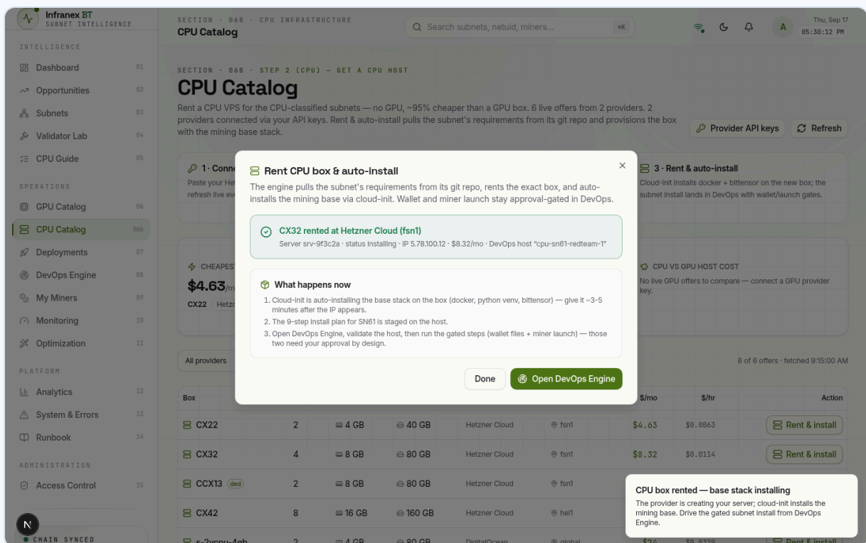
Figure 7. The success panel — example data. "CX32 rented at Hetzner Cloud (fsn1)" with server id, IP, price and the DevOps host name, plus the "What happens now" list and a shortcut into DevOps Engine.
