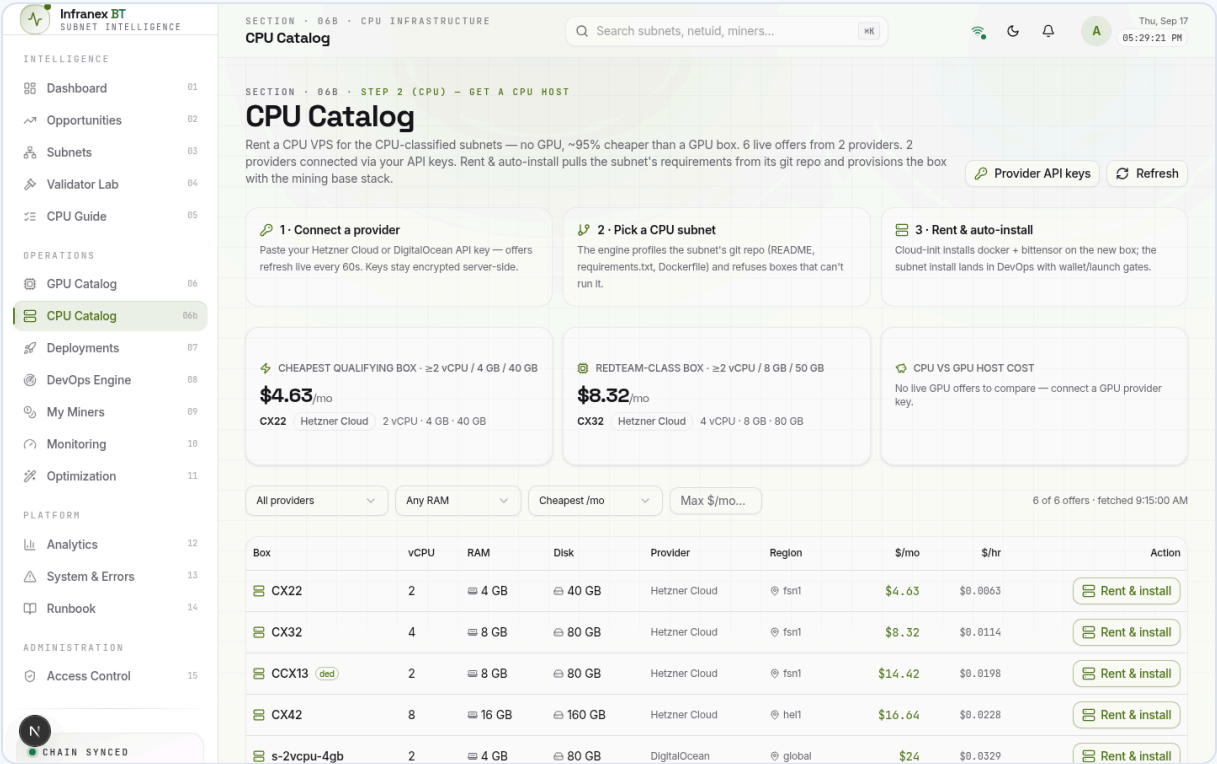
Figure 5. The catalog with a connected key — example data (a representative Hetzner + DigitalOcean snapshot). With your own key you will see your real, live prices in this exact layout.
