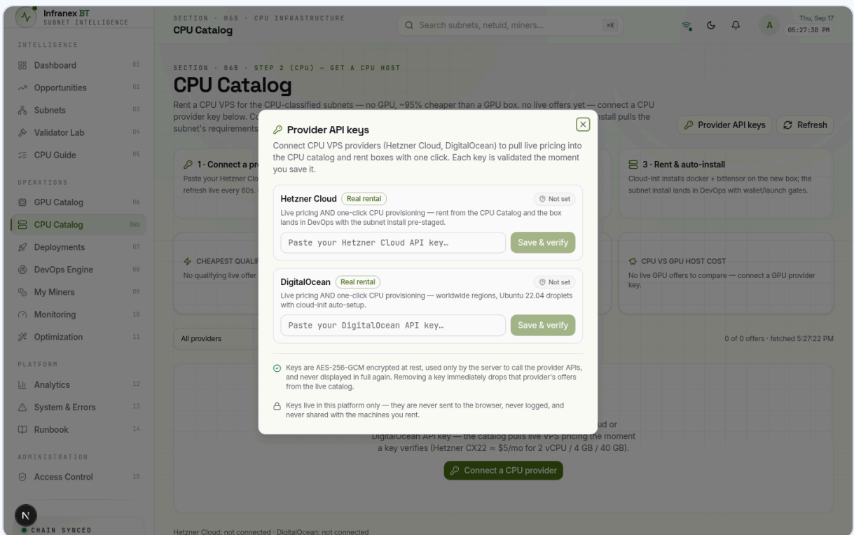
Figure 3. The Provider API keys dialog in its CPU mode: Hetzner Cloud and DigitalOcean, each with a paste field and a Save & verify button. Status pills show whether a stored key is valid.
