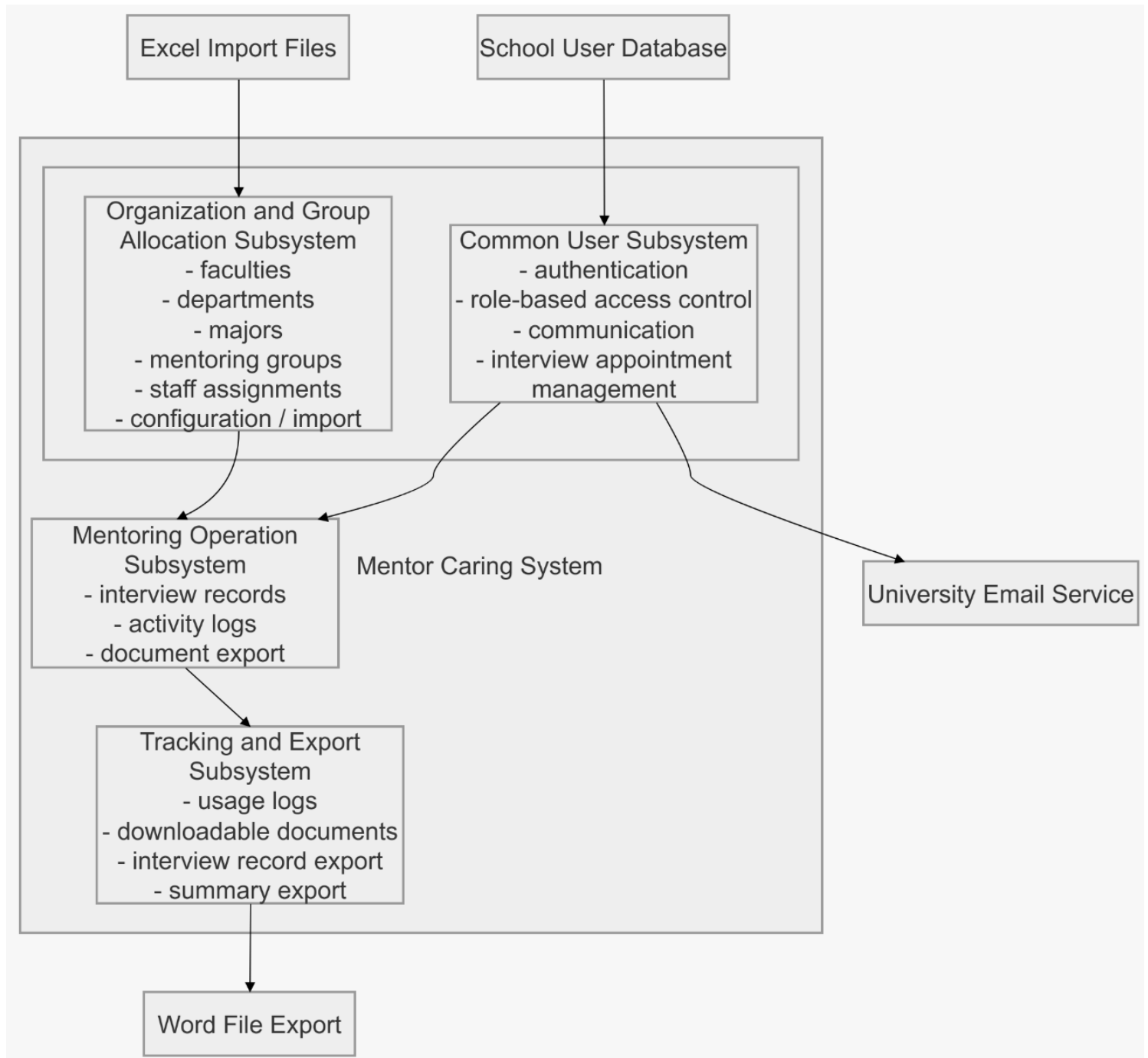
Figure 4: System architecture of the Mentor Caring System
