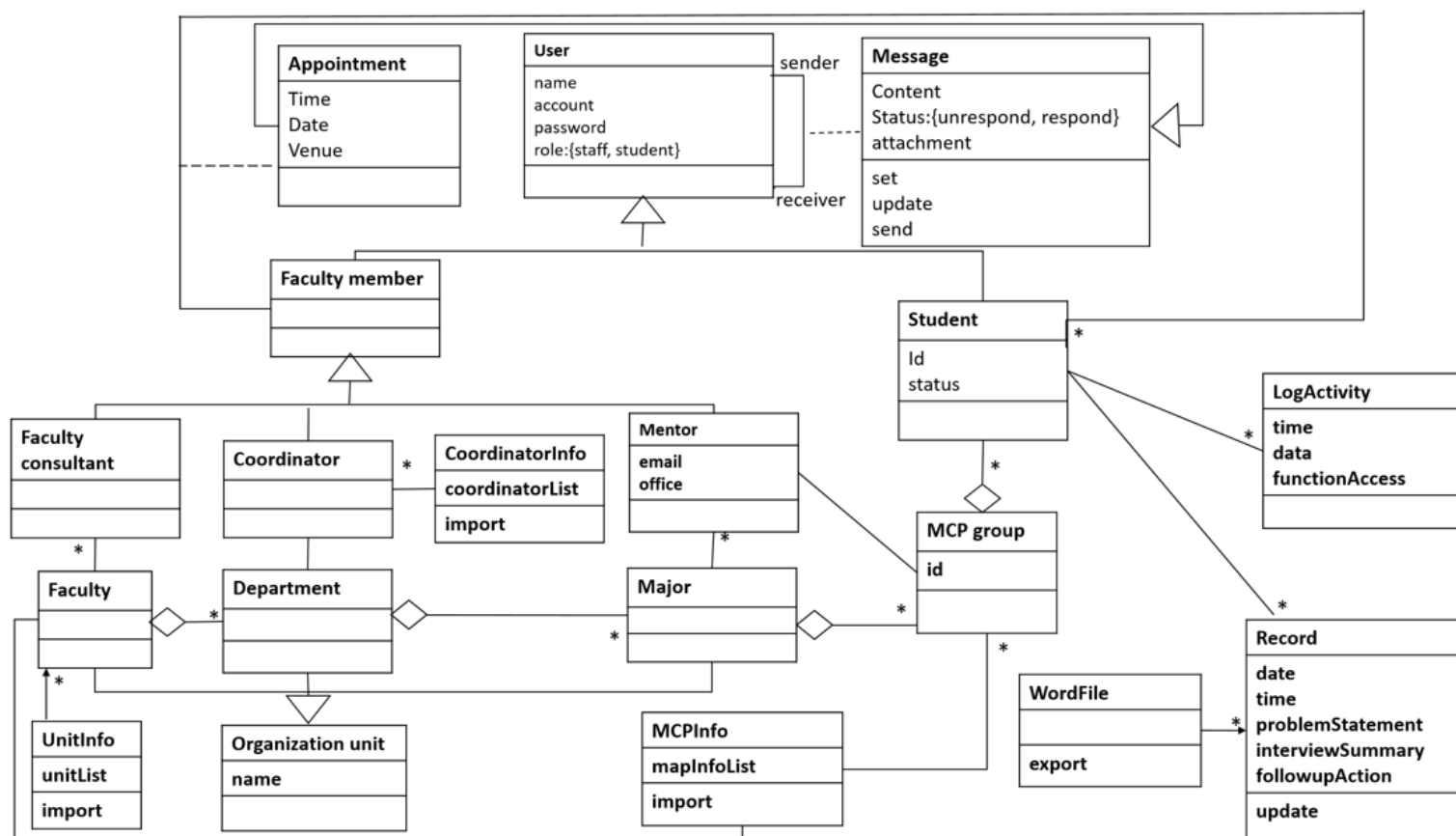
Figure 1: Class Diagram of the Mentor Caring System
