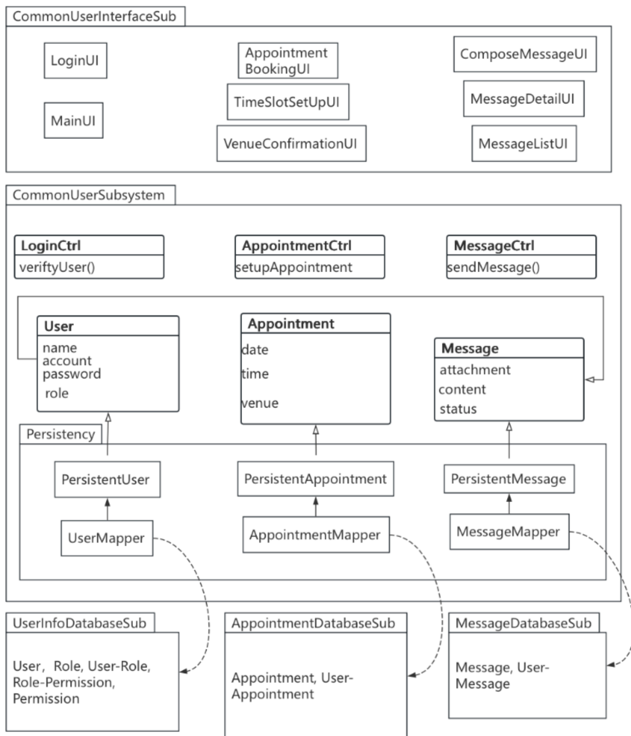
Figure 5: Architecture diagram of the Common User Subsystem
