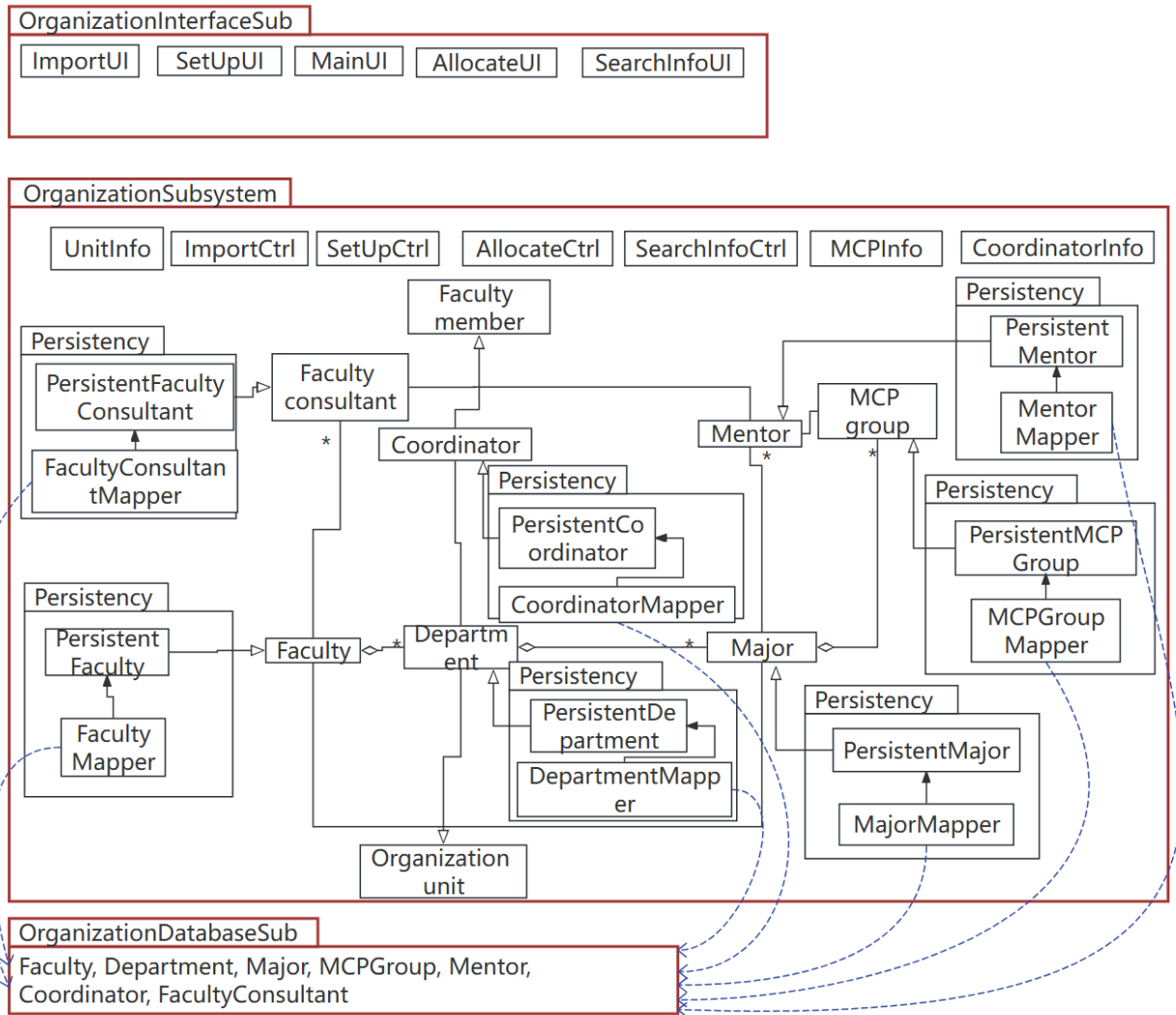
Figure 7: Architecture diagram of the Organization and Group Allocation Subsystem
