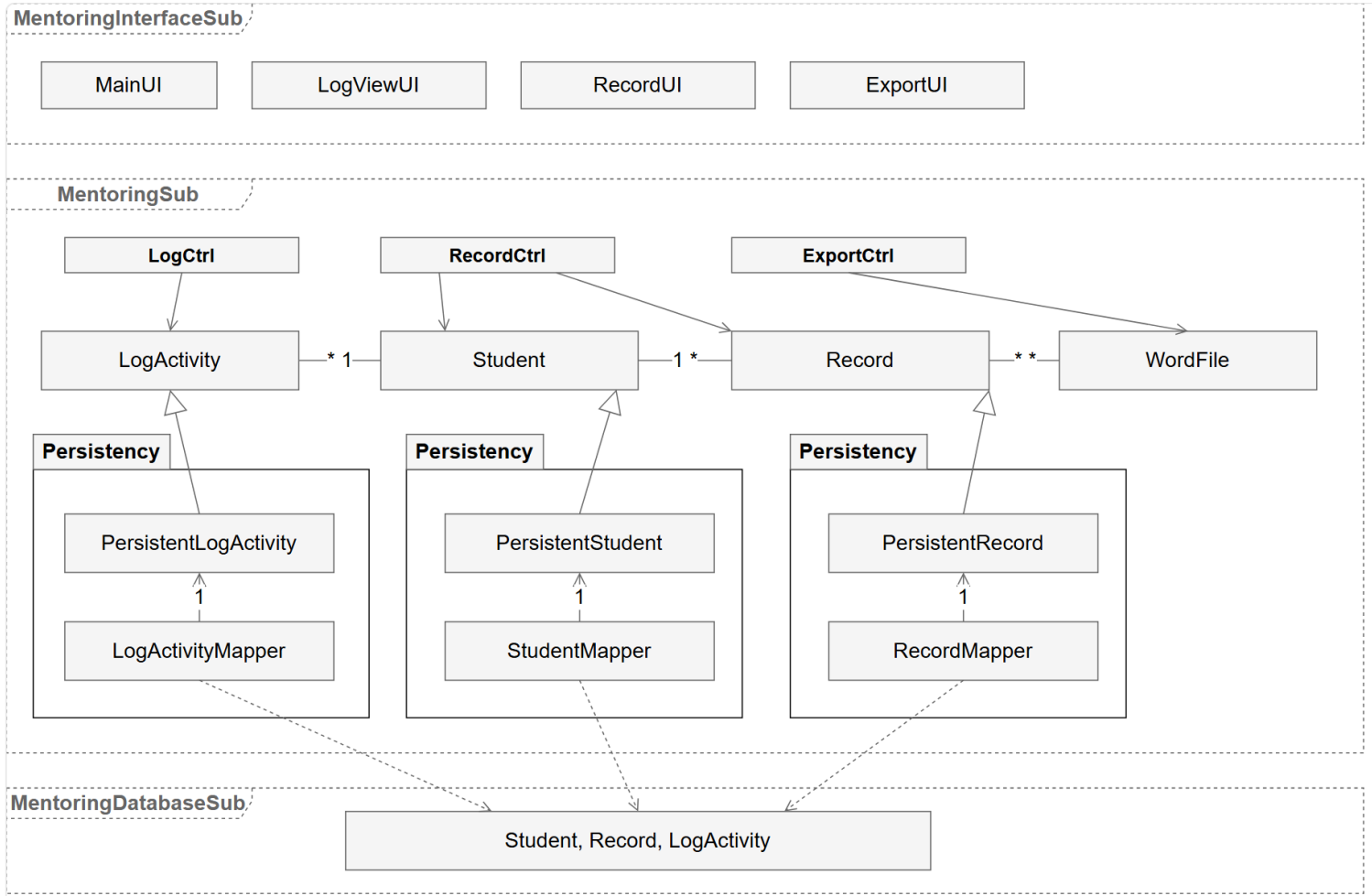
Figure 8: Architecture diagram of the Mentoring Operation Subsystem
