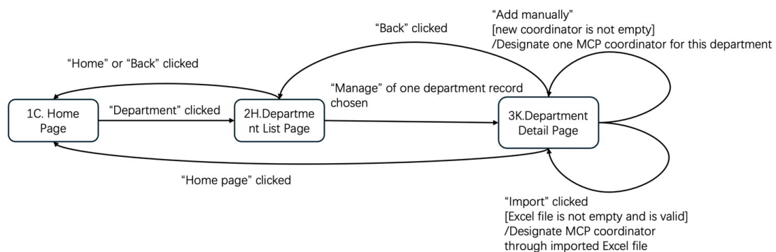
Figure 8: Designate Coordinators
