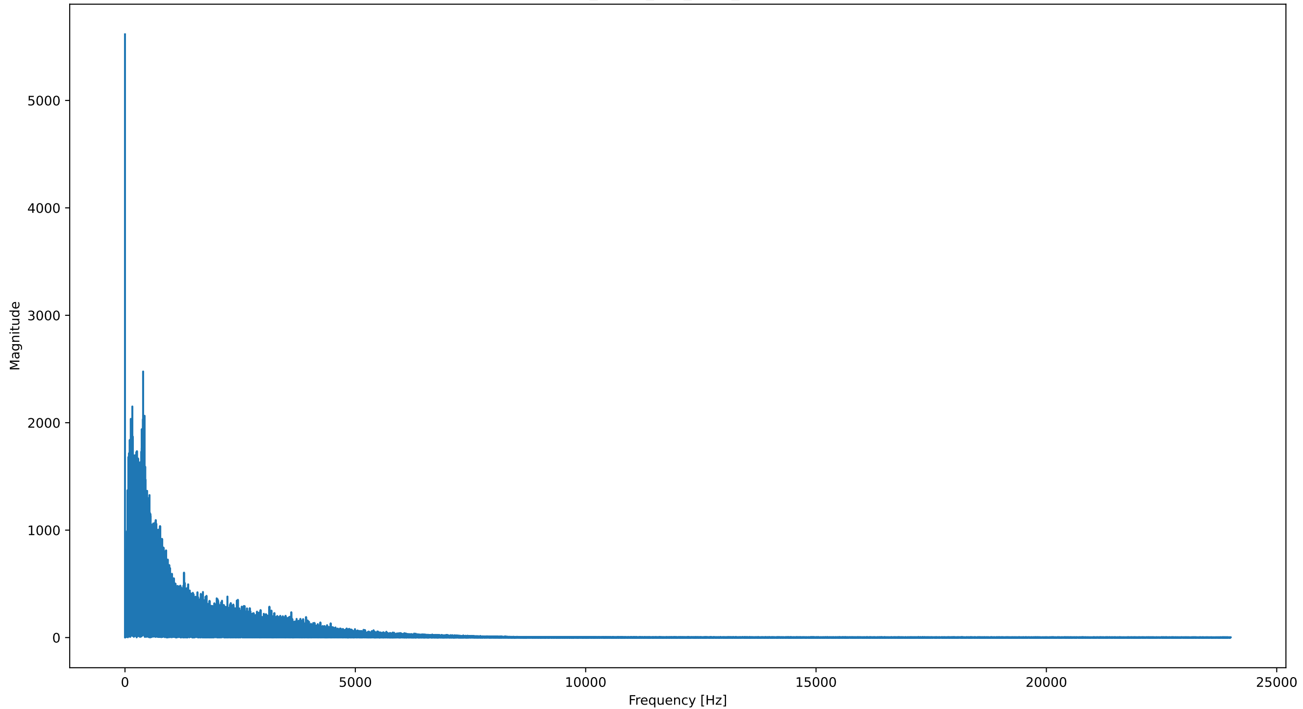
Aircraft audio A5-0001_OPT G_002_0001_Tr1 - Magnitude Spectrum
