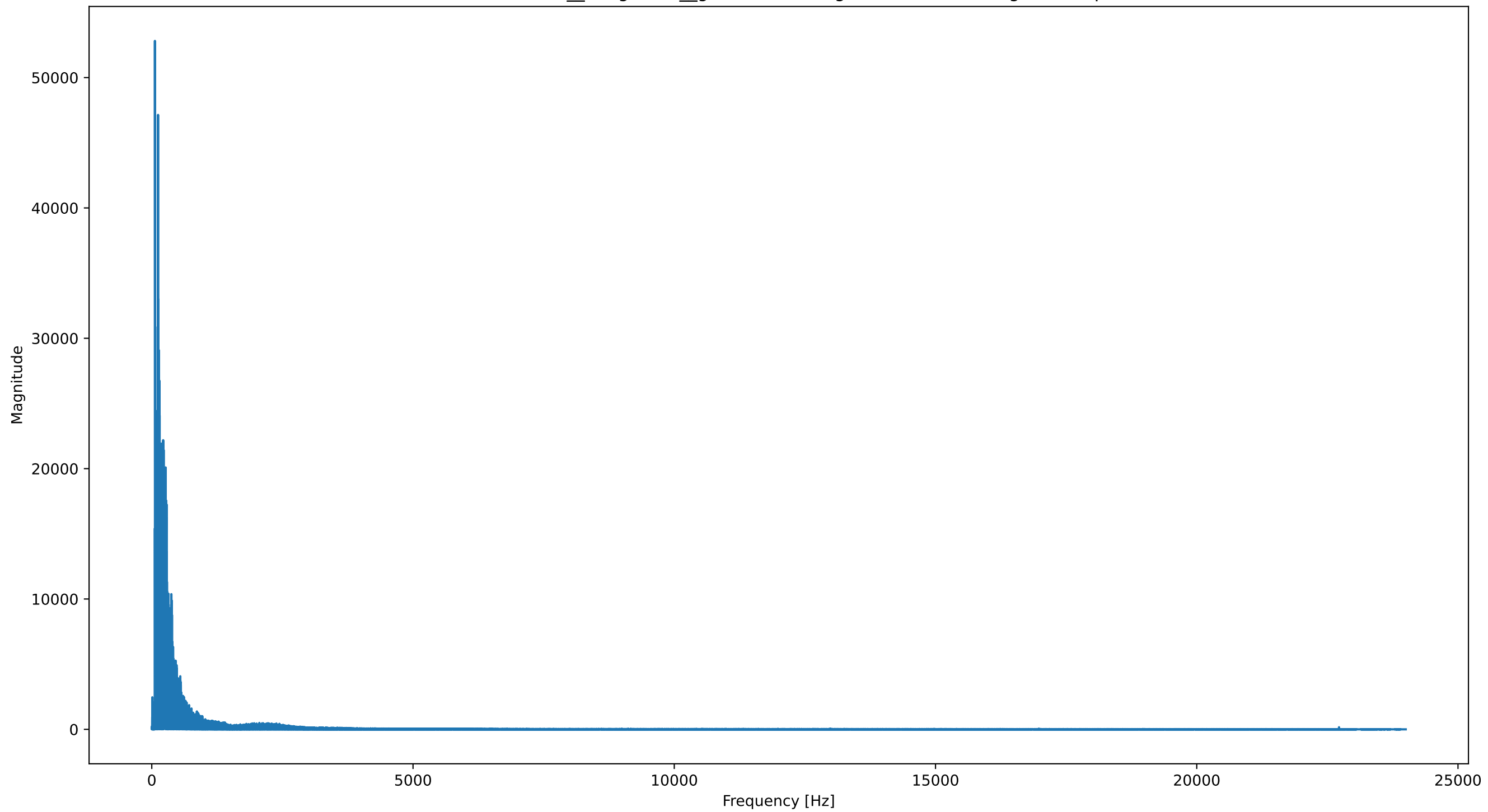
Noise audio 438866__craigsmith__g55-12-moaning-whistle-wind - Magnitude Spectrum
