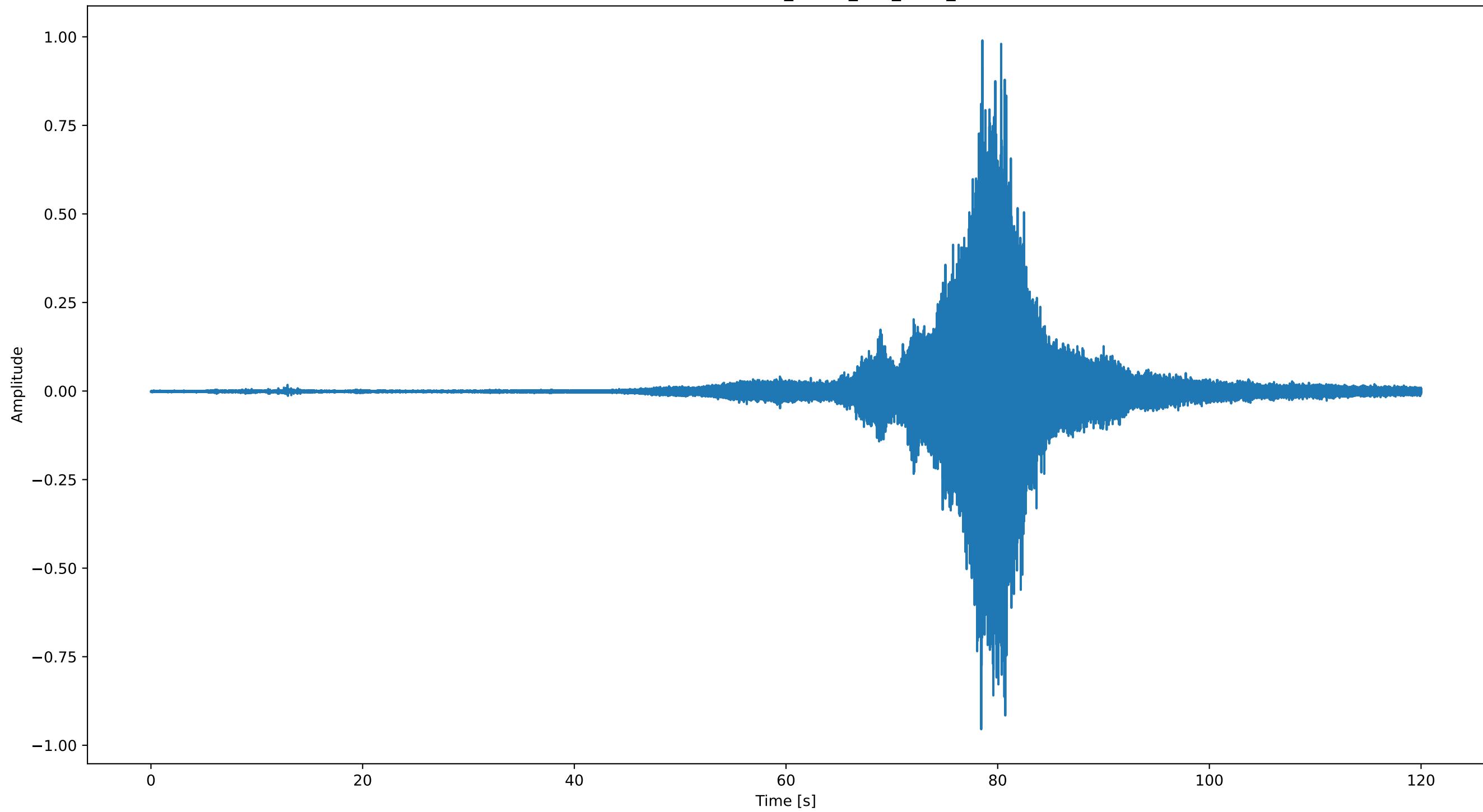
Waveform of aircraft audio A5-0001_OPT G_002_0001_Tr1 1 - Waveform
