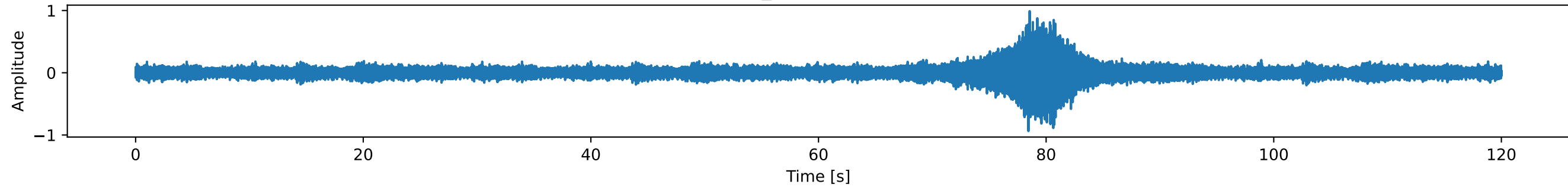
Mixture_snr5 4 - Waveform
