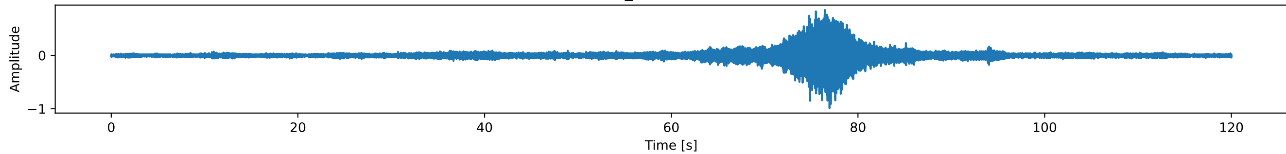
Mixture_snr5 2 - Waveform
