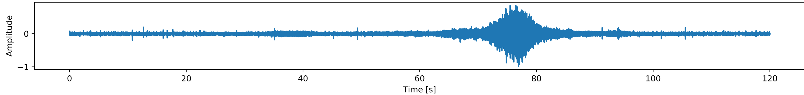
Mixture_snr5 3 - Waveform
