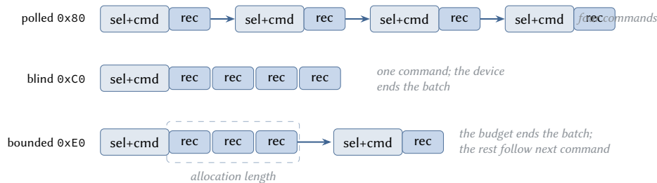
Figure 1: Four frames queued. Polled mode pays a fresh arbitration and selection per record. Blind mode takes all four in one command, the device deciding where the batch ends. Bounded mode takes as many as the allocation length allows and leaves the rest for the next command.
