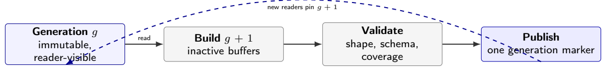
Figure 2: Copy-publish generations keep readers on immutable state while the next coherent set of slices is assembled.
