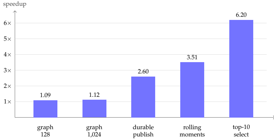
Figure 6: Central-estimate speedup against the matched pre-change or reference lane. The first three are before/after Hypercube results; the final two compare algorithms in the same current harness.
