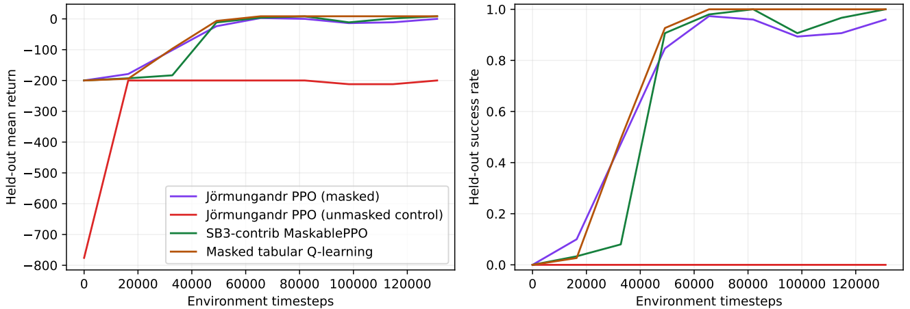
Figure 8: Taxi-v4 return and task-completion learning curves. Every masked participant uses the environment-supplied mask; the red control alone may select masked actions. Curves are means across three training seeds.
