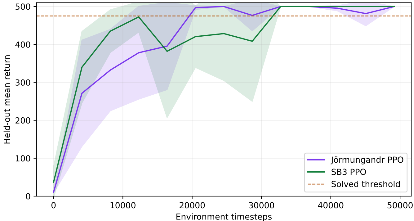
CartPole-v1 PPO implementation diagnostic
