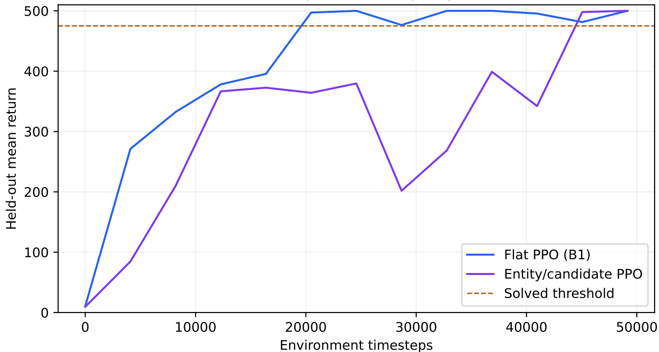
CartPole representation parity (S0)
