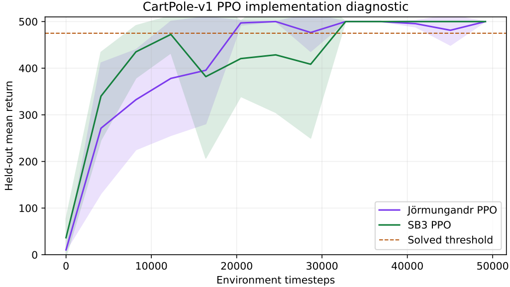
Figure 5: Matched-capacity CartPole PPO diagnostic. Lines are the mean of three independent training seeds and shading is one standard deviation of the three held-out run means. The curve is a wiring benchmark, not a library-wide performance ranking.
