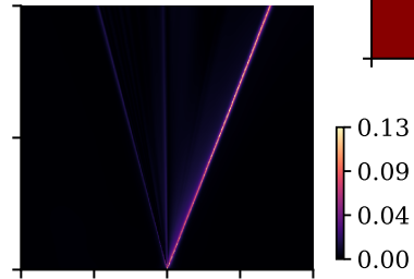
(e) TRG-PINN error ( p )
