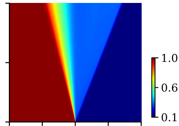
(c) TRG-PINN ( p )
