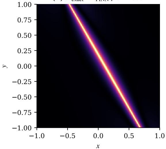
(a) |u_{\text{exact}} - u_{\text{PINN}}| , t = 0.5
