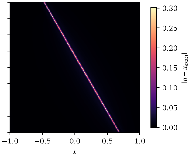
(b) |u_{\text{exact}} - u_{\text{TRG-PINN}}| , t = 0.5
