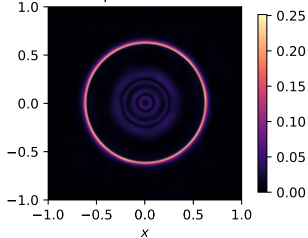
PINN pointwise RMSE
