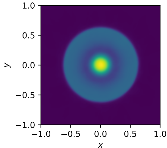
PINN median h
