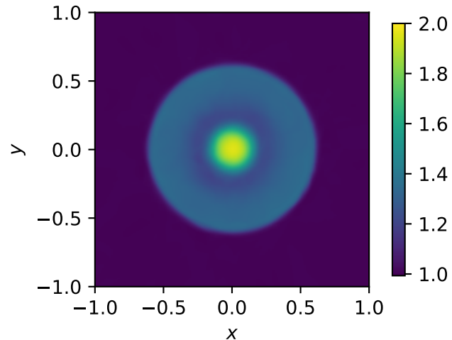
TRG-PINN median h
