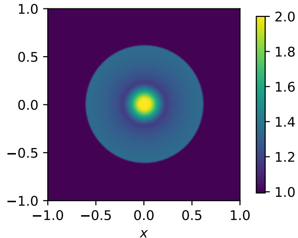
FV reference h
