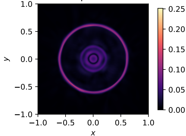
TRG-PINN pointwise RMSE
