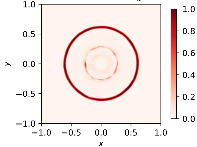
TRG-PINN median gate
