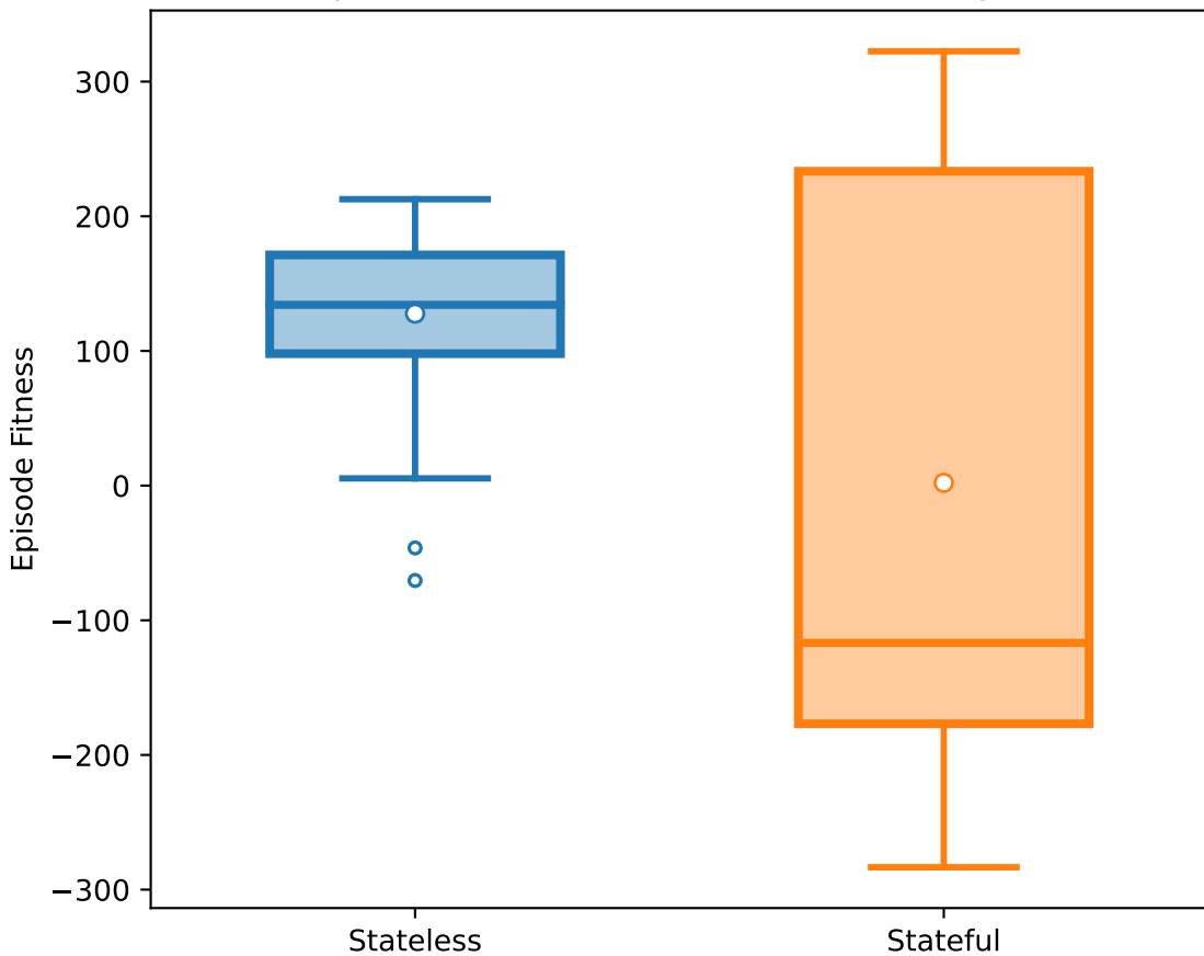
Episode Fitness with Indistribution Targets
