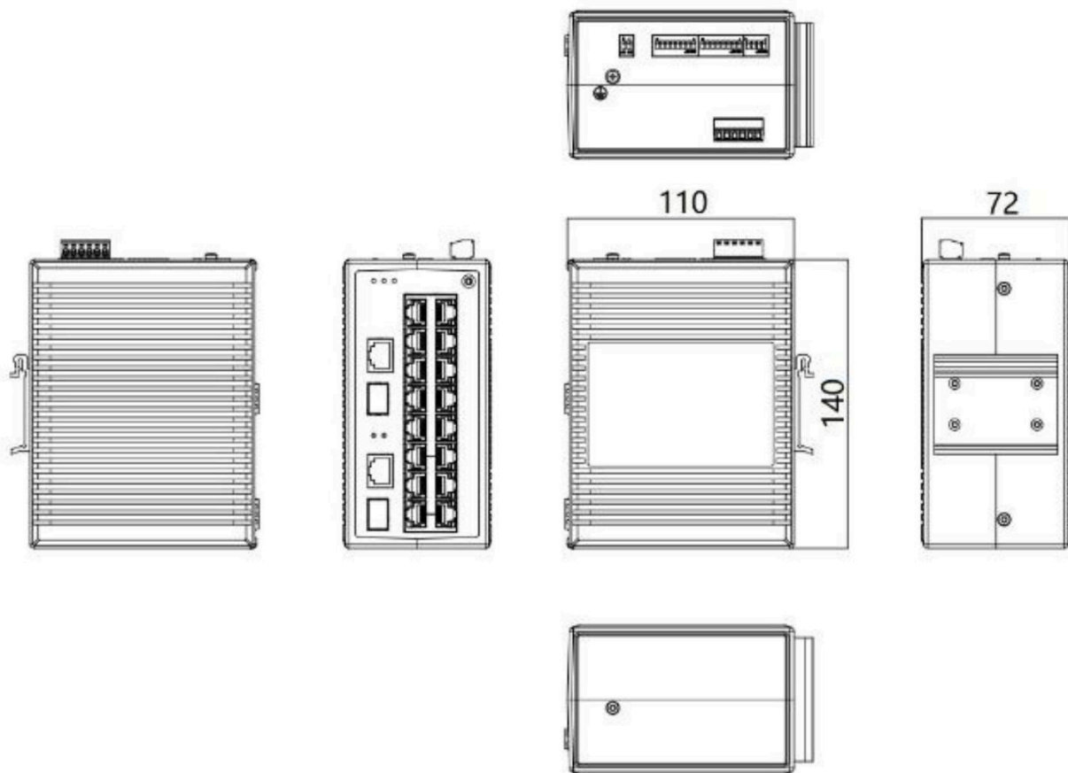
Dimension Diagram
