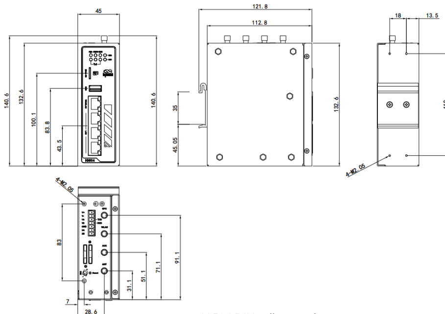
IG504 DIN-rail mounting
