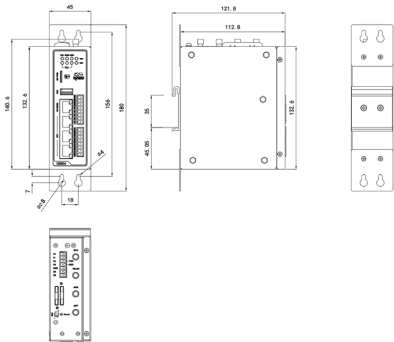
IG504 wall mounting
