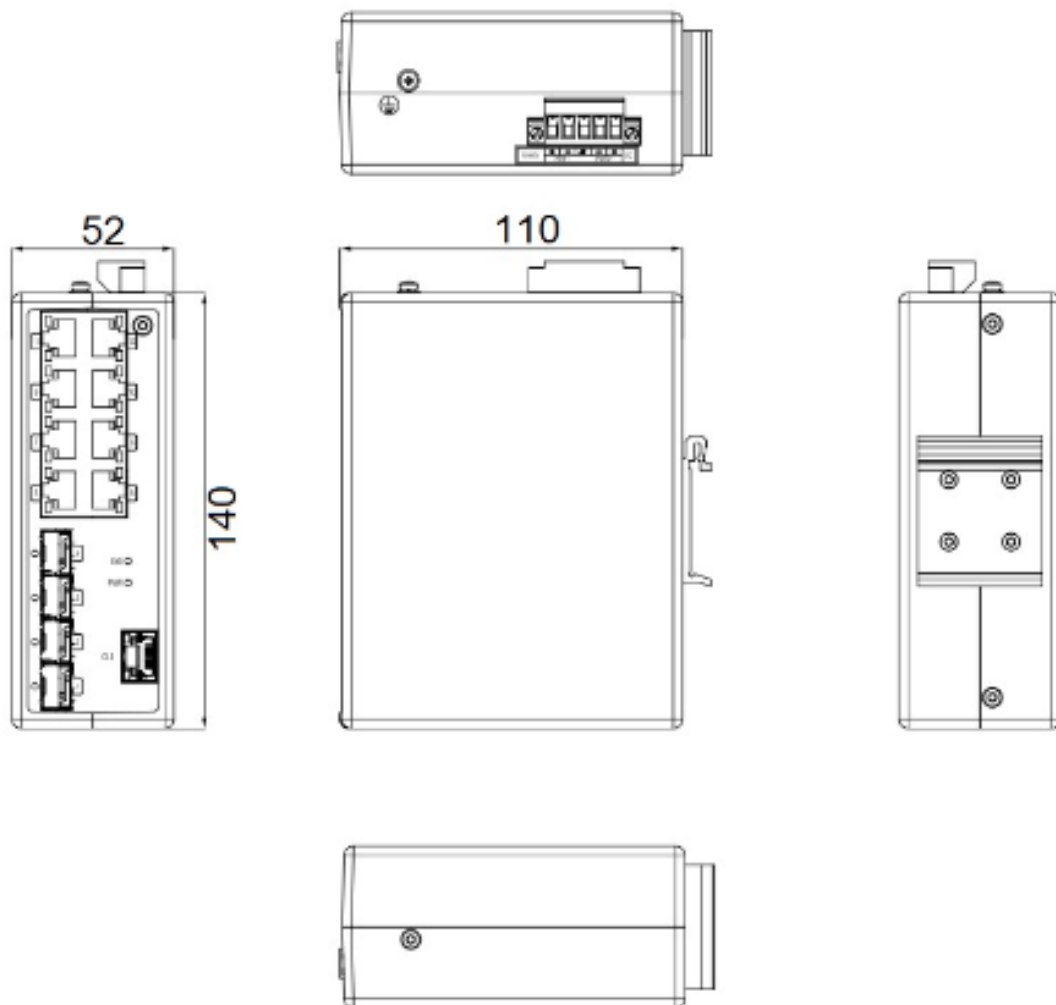
ISM7012D-P (52 × 140 × 110 mm (2.05 × 5.51 × 4.33 in))
