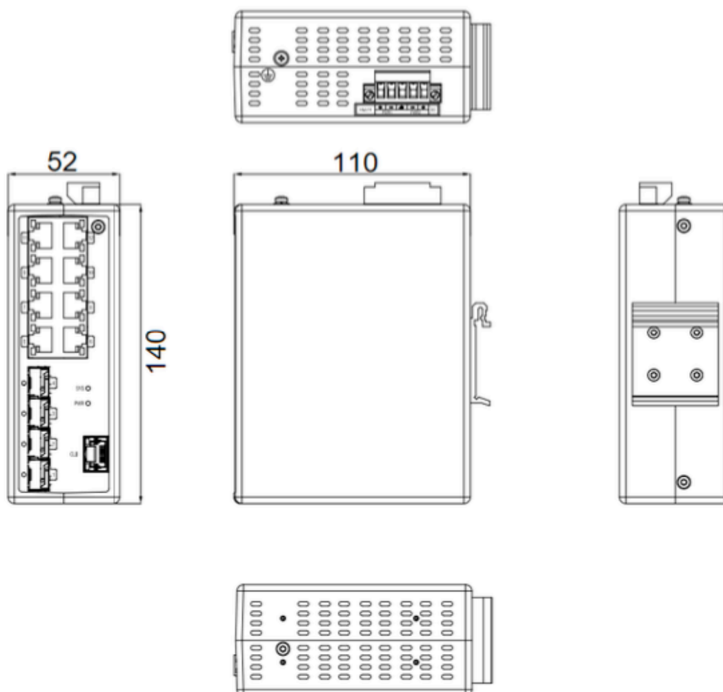
ISM7312D (52 × 140 × 110 mm (2.05 × 5.51 × 4.33 in))
